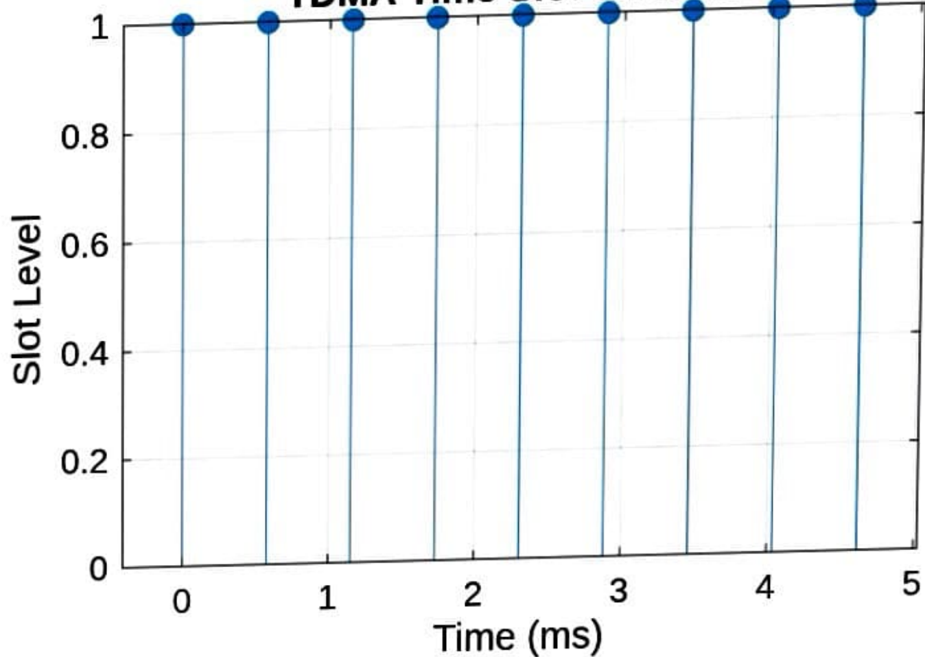
TDMA Time Slot Structure
